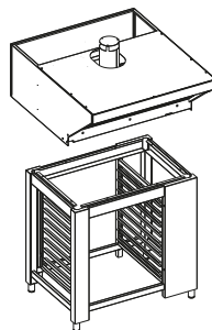
BASE CON PORTATEGLIE E CAPPA BASE WITH TRAY RACK AND HOOD
